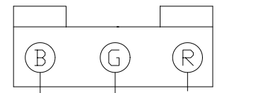
End View of 3-Pin MOLEX connector
